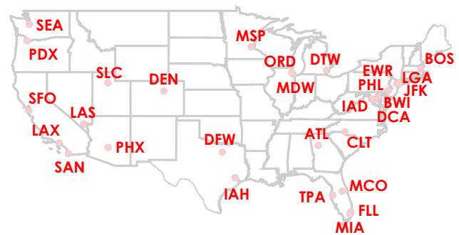
Fig. 10. Geographic locations of the US airports considered in our analysis (IATA code given). Note that HNL is not shown for simplicity.
