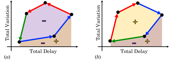
Fig. 4. A DRT where higher TV is associated with recovery (left), and a DRT where higher TV is associated with disruption (right).
