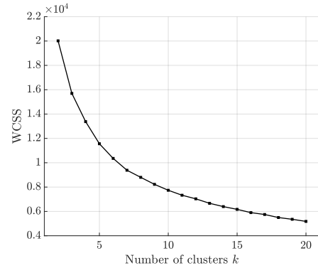
Fig. 6. Within cluster sum-of-square (WCSS) error versus the number of clusters.
