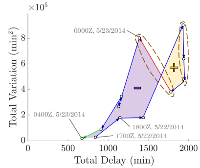
Fig. 2. A 12-hour long DRT transitions out of the nominal region at 1700Z. Arrows denote maneuvers, and their colors denote the succeeding region (see Figure 1). Select DRT features from Section II-E such as signed enclosed area and trade-off maneuvers (brown dashed indicators) are annotated. Note that each state is a one hour interval.
