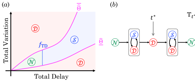
Fig. 1. (a) A disjoint partition of the TV-TD state space into three regions; (b) Schematic representation of a disruption-recovery trajectory \mathbb{T}_{t^*} constructed via Algorithm 1 anchored in time at t^* .
