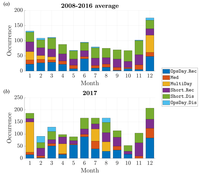
Fig. 8. Occurrence counts of DRT hours for each month, split by representative DRT clusters; counts (a) averaged across 2008-2016 and (b) for 2017.
