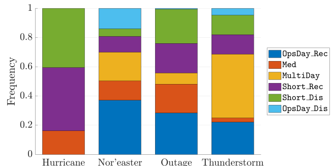
Fig. 7. Frequency of representative DRTs, given the occurrence of an off-nominal event. The extreme Dec08Event cluster is not shown.
